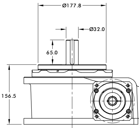
Shaft Output
